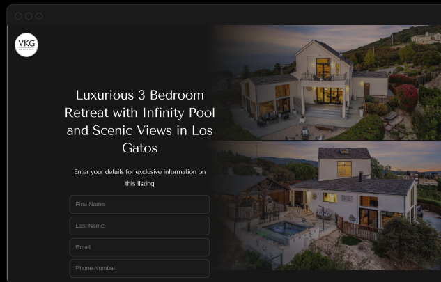
Landing Page
