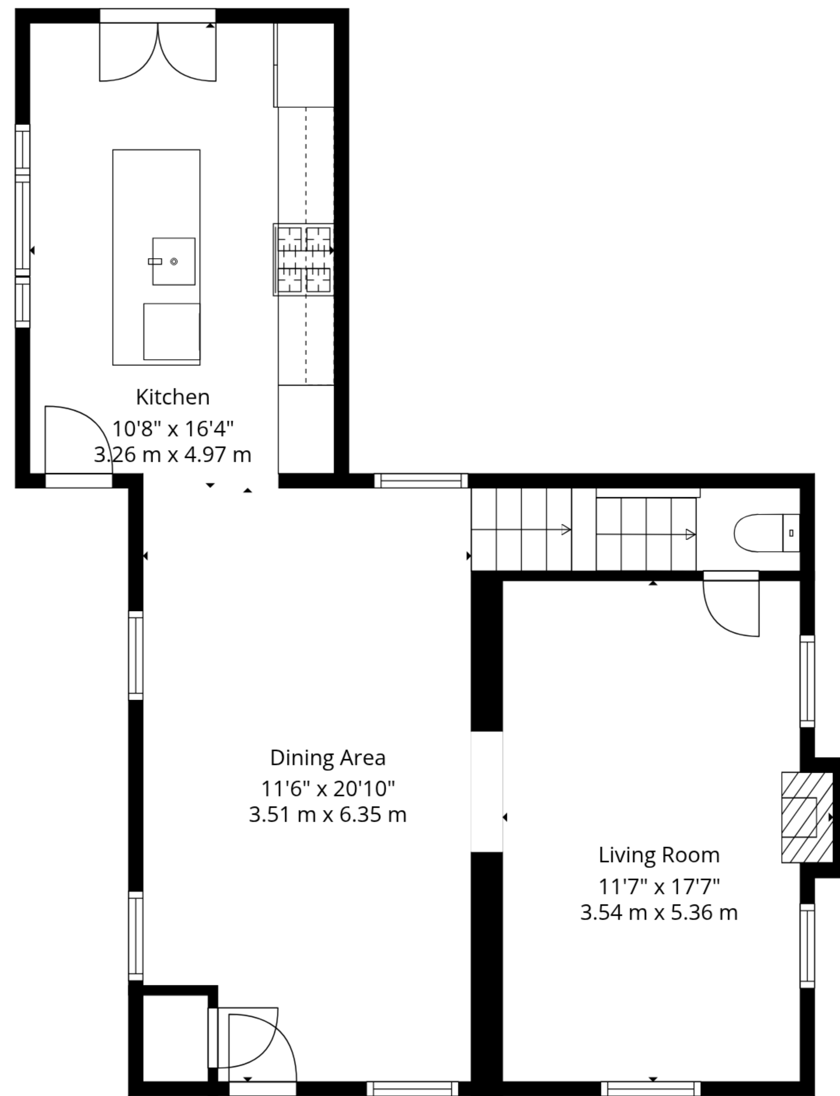
1st Floor
