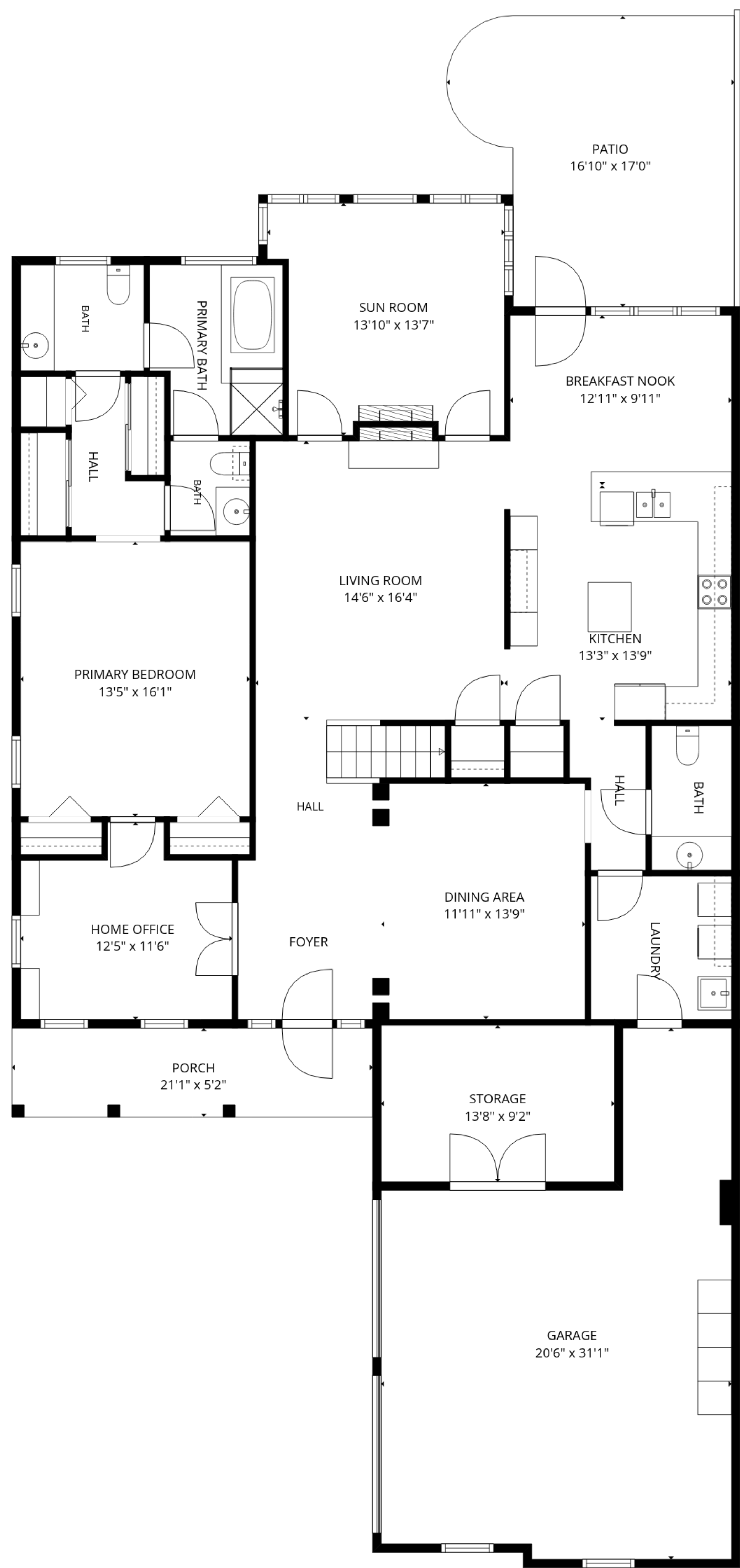
1st floor
