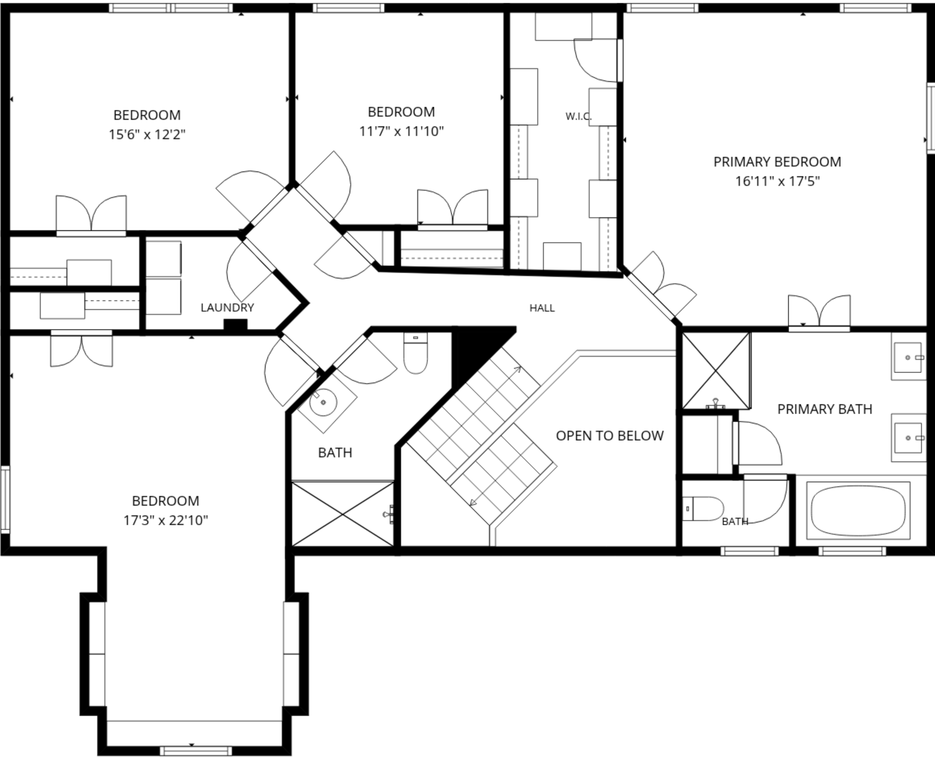
2nd floor
