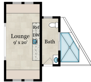
POOL CABANA 270 SQ FT
