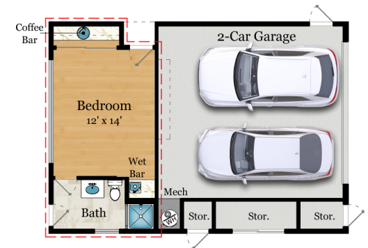
GUEST UNIT/DETACHED GARAGE
