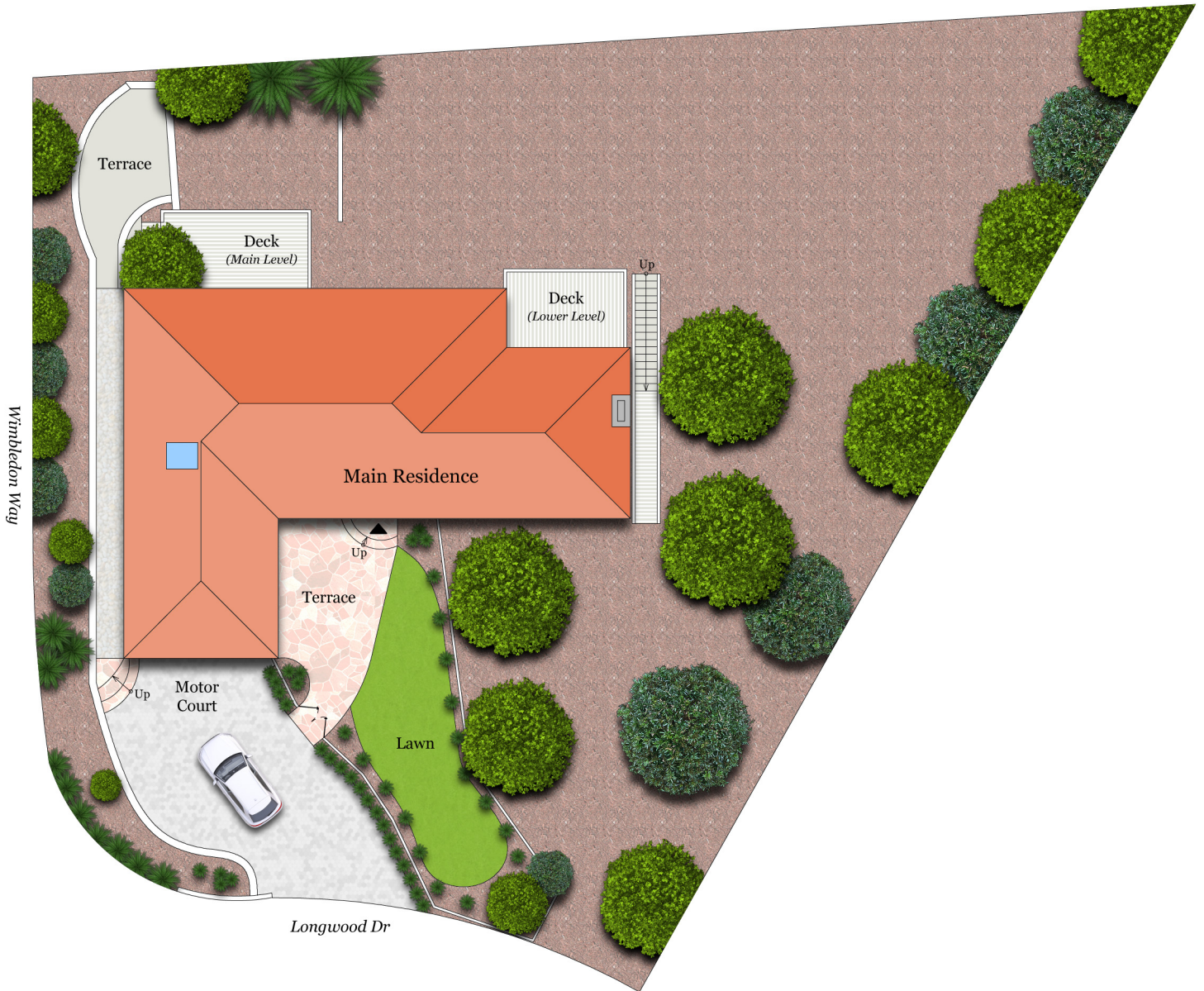
SITE PLAN
