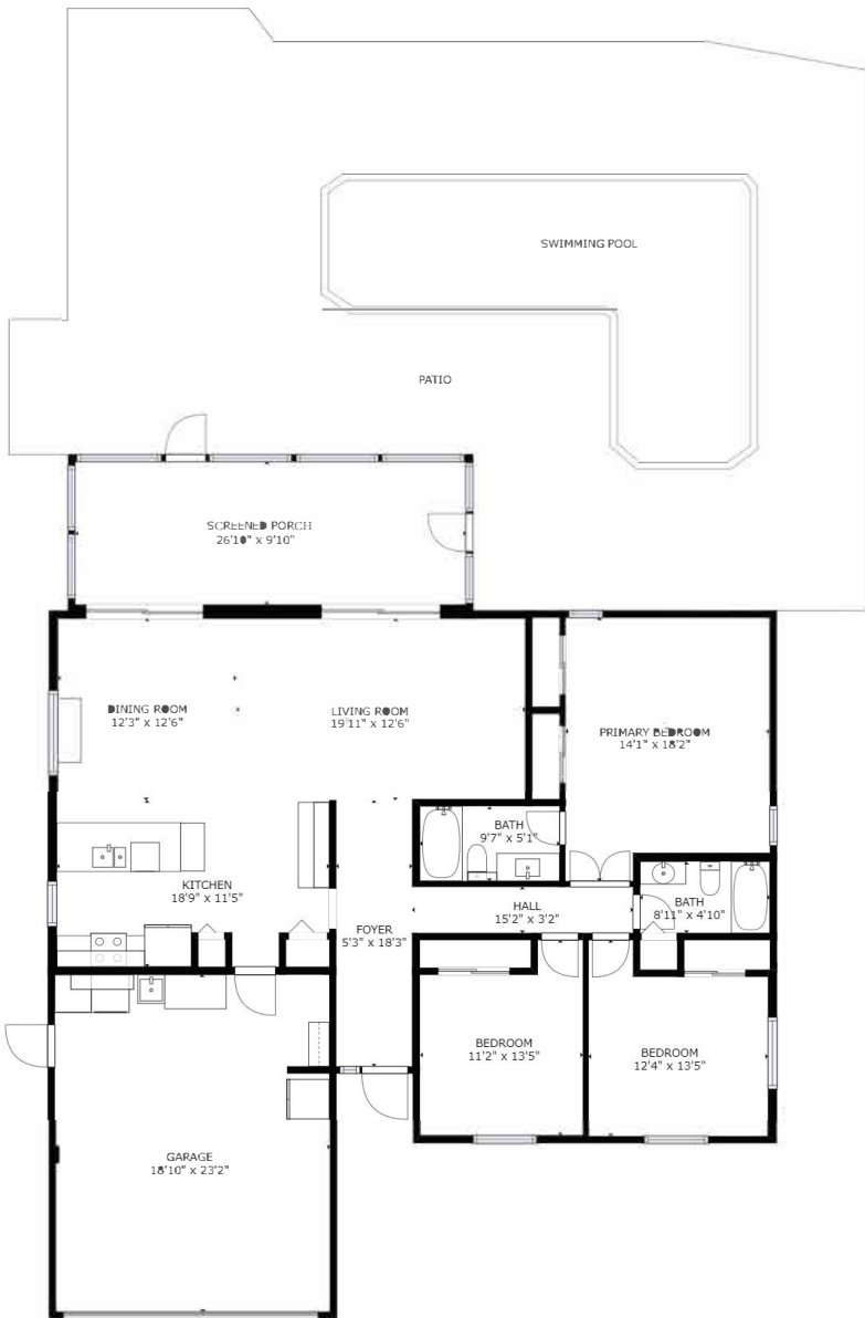
FLOOR 1
