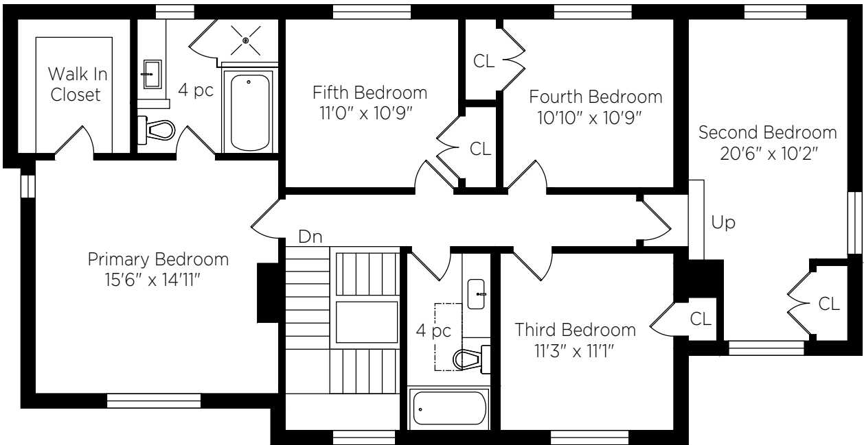
Second Floor 1410 Square Feet
