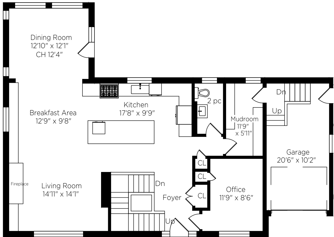
Main Floor 1270 Square Feet + 246 Garage
