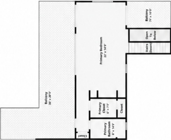
GUEST HOUSE FLOOR 2
