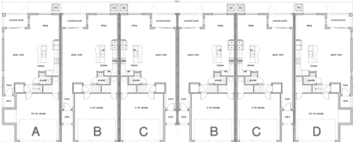
OVERALL FIRST FLOOR PLAN
