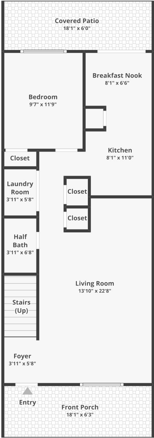
FLOOR 1
