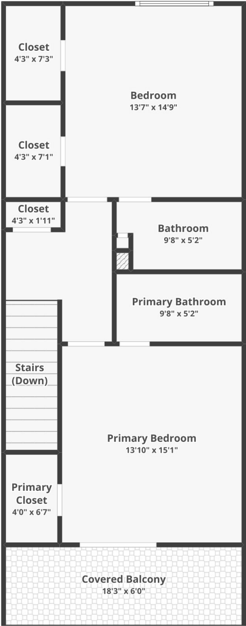
FLOOR 2
