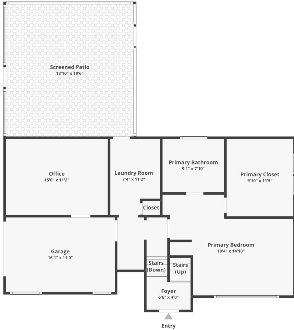
FLOOR 1
