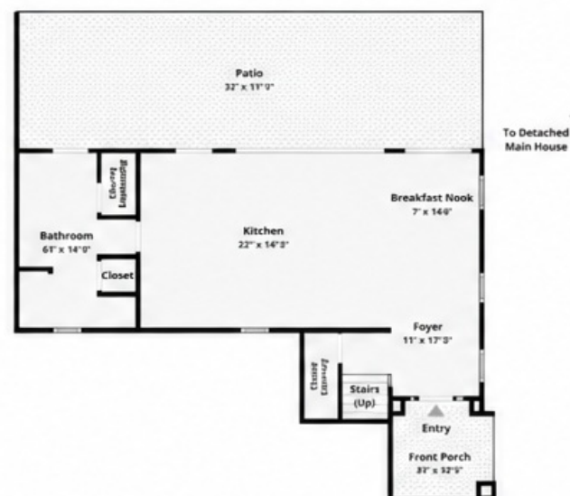
GUEST HOUSE FLOOR 1
