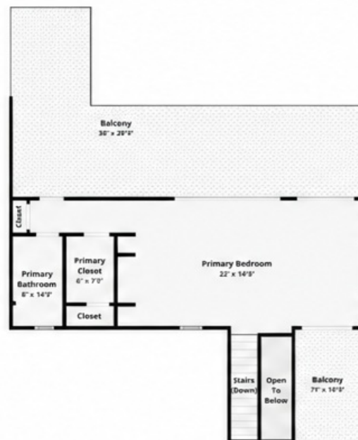
GUEST HOUSE FLOOR 2
