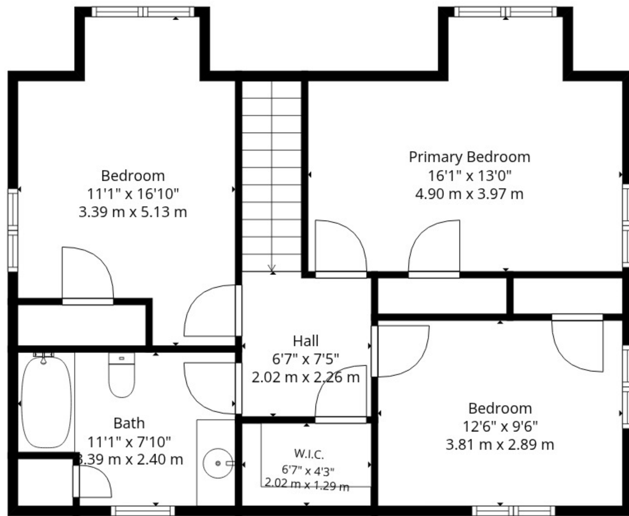
Main Cottage Upper Level
