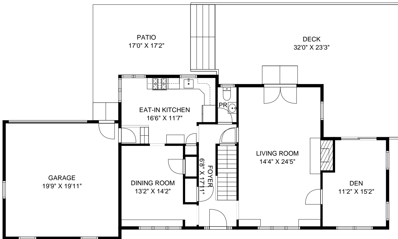
FIRST FLOOR
