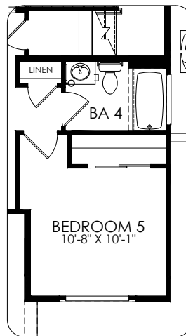
70030 - Bedroom and Bath
