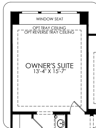
70241 - Window Seat
