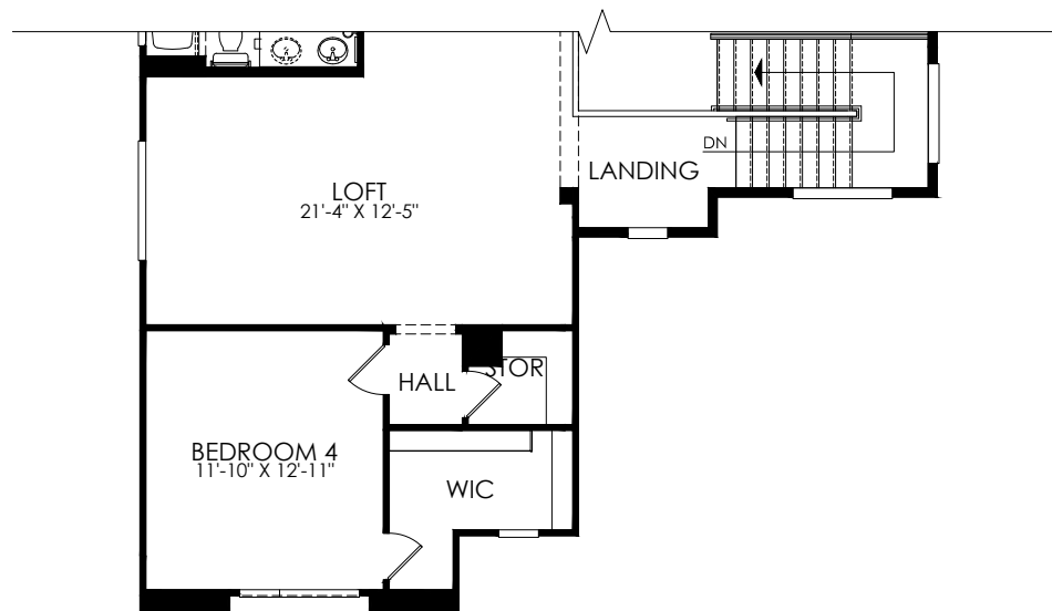
Second Floor Plan - Elevation 'C'
