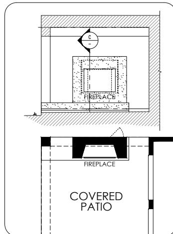
70840 - Fireplace Exterior 2
