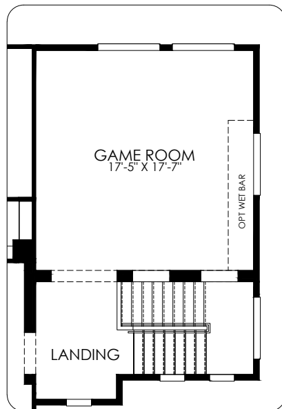
70094 - Game Room
