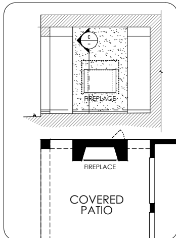
70838 - Fireplace Exterior
