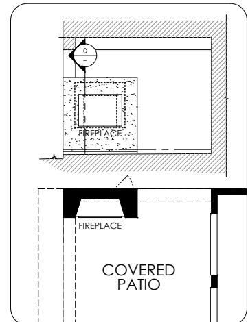
70846 - Fireplace Exterior 3
