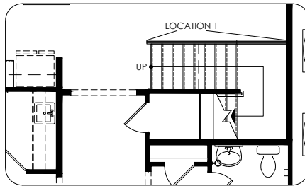
Stair Rail - Location 1
