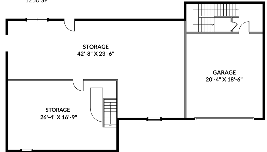
LOWER LEVEL 75 SF
