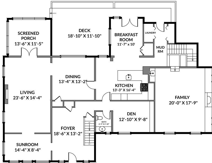
FIRST FLOOR 2140 SF
