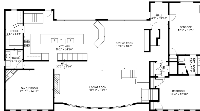
FLOOR 1
