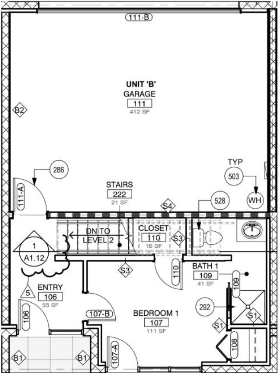
UNIT "B" LEVEL ONE FLOOR PLAN
