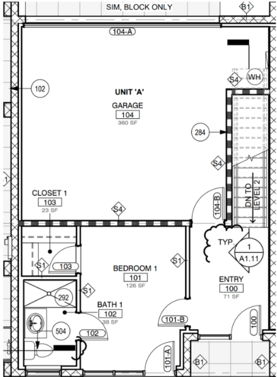
UNIT "A" LEVEL ONE FLOOR PLAN
