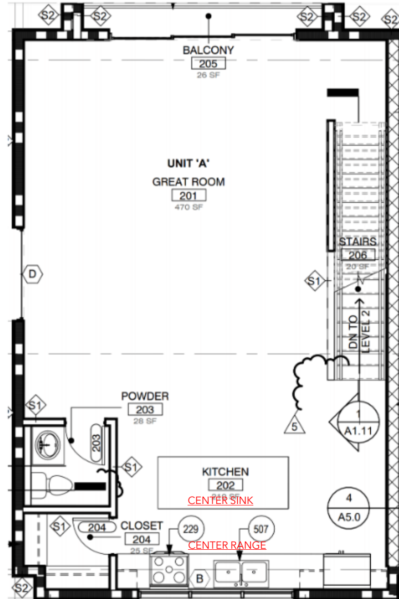
UNIT "A" LEVEL TWO FLOOR PLAN
