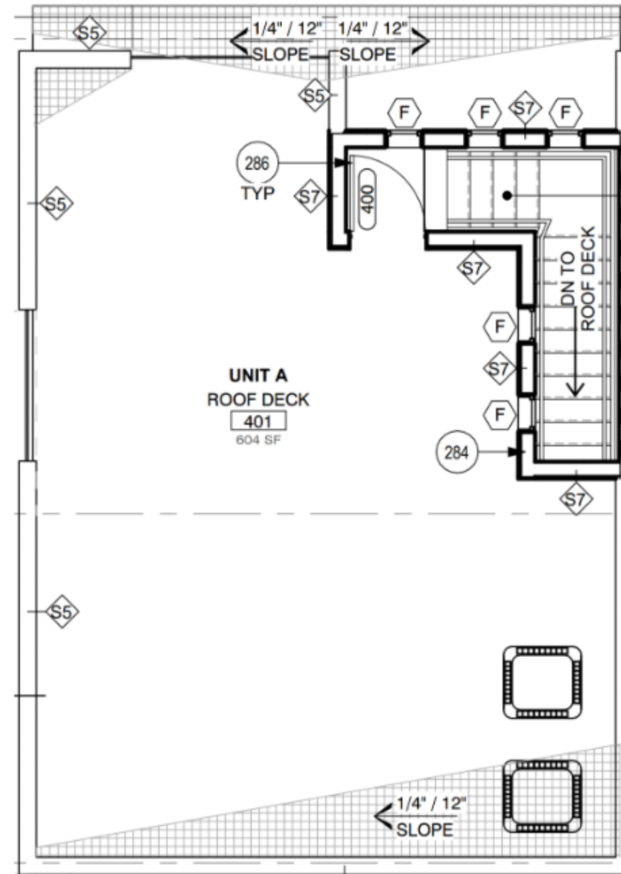
UNIT "A" LEVEL FOUR FLOOR PLAN
