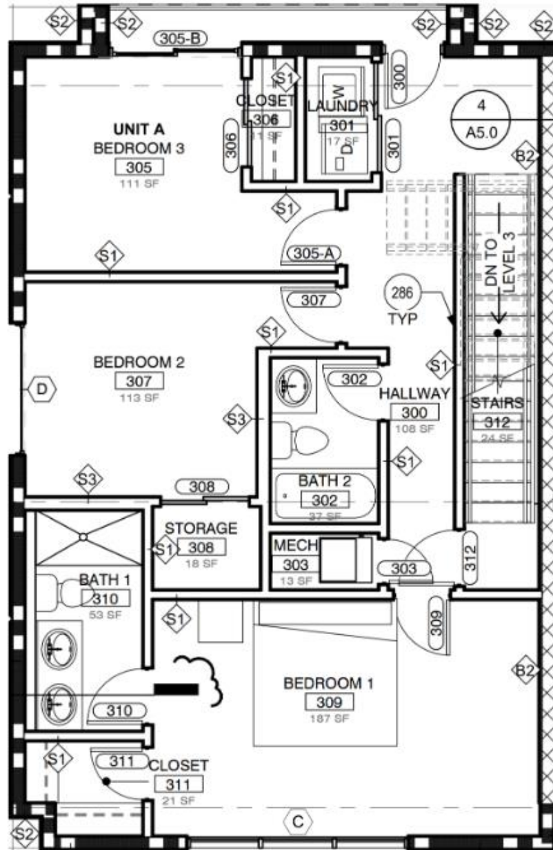
UNIT "A" LEVEL THREE FLOOR PLAN
