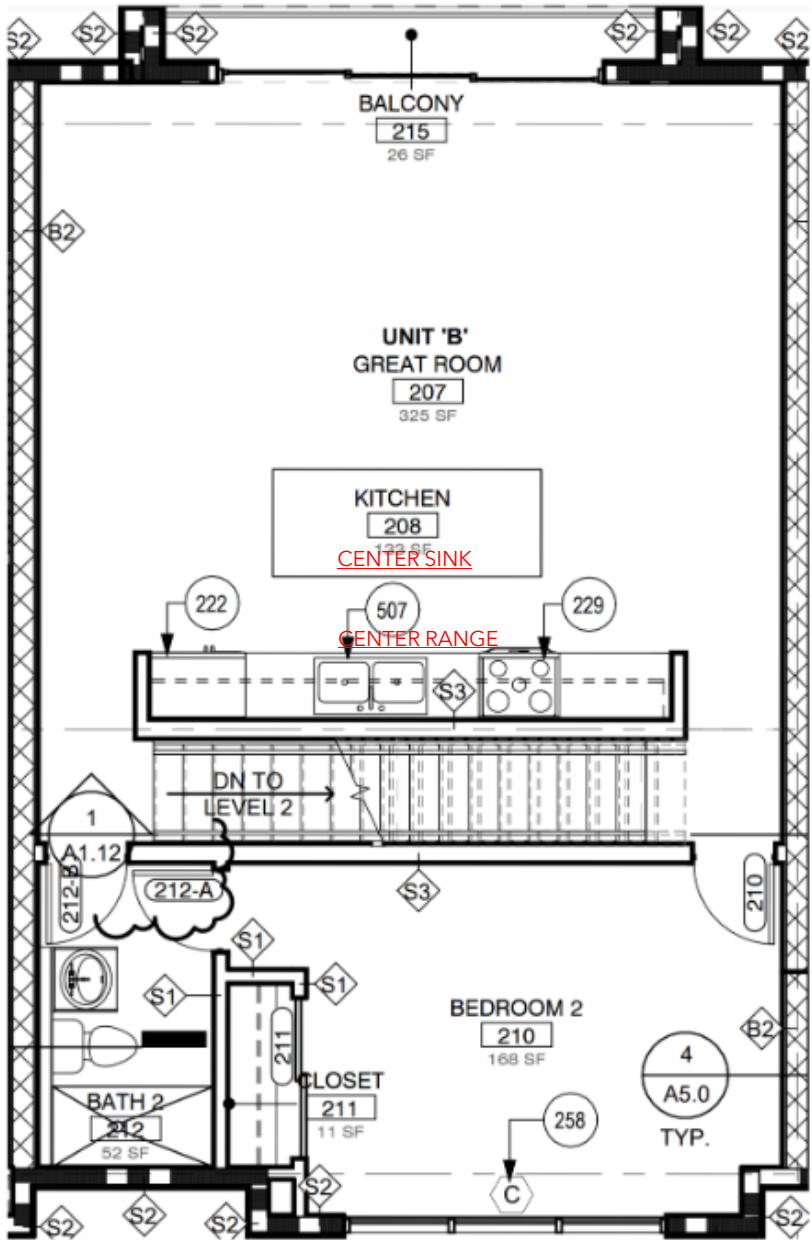
UNIT "B" LEVEL TWO FLOOR PLAN
