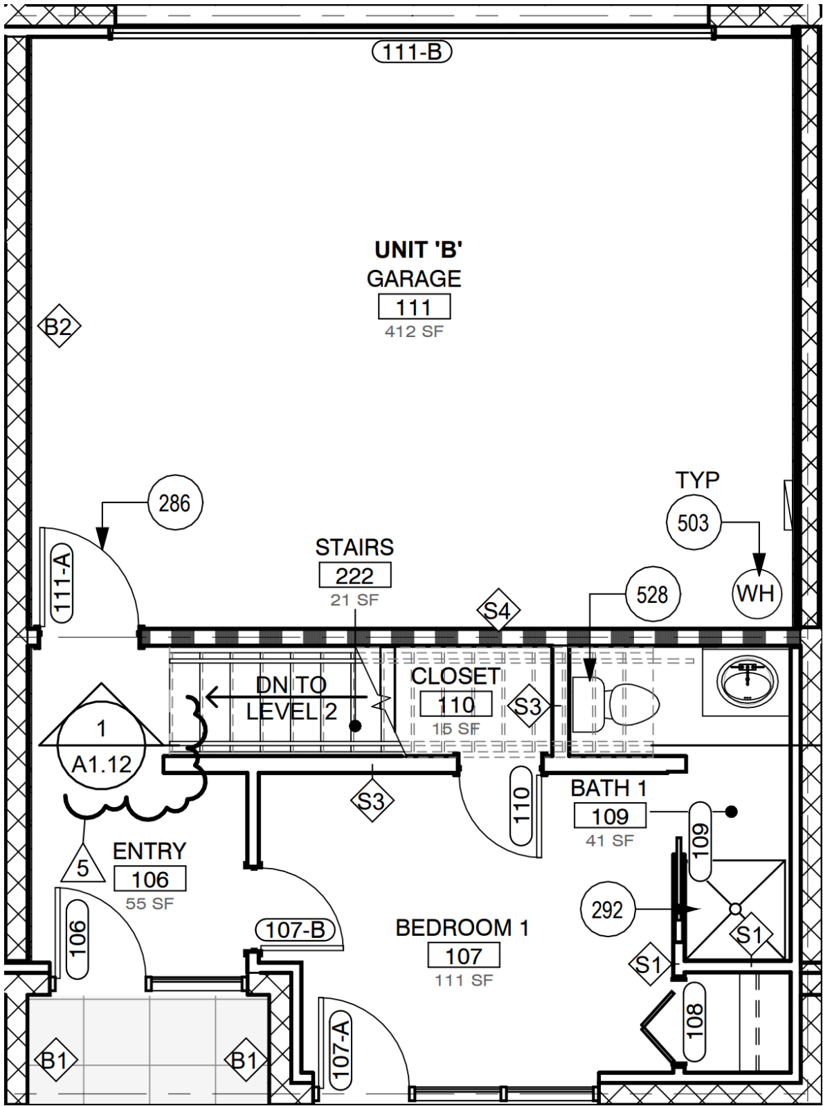
UNIT "B" LEVEL ONE FLOOR PLAN
