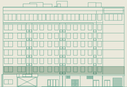
NORTHWEST ELEVATION
