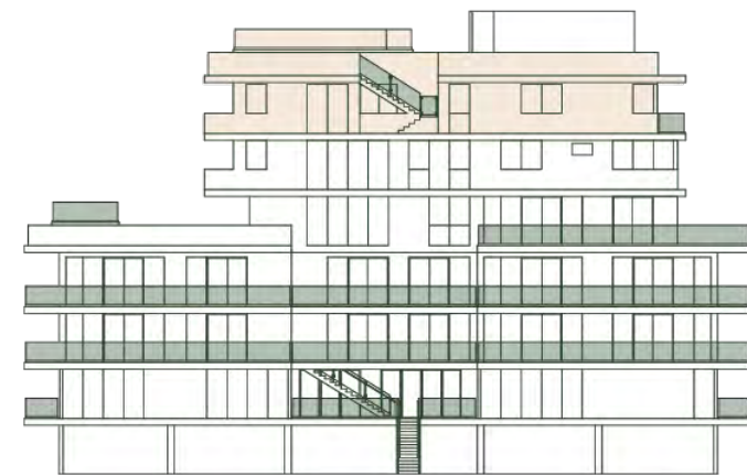
EAST FACADE
