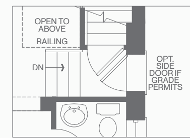
PARTIAL GROUND FLOOR PLAN W/OPT. SIDE DOOR ELEVATION A, B + C
