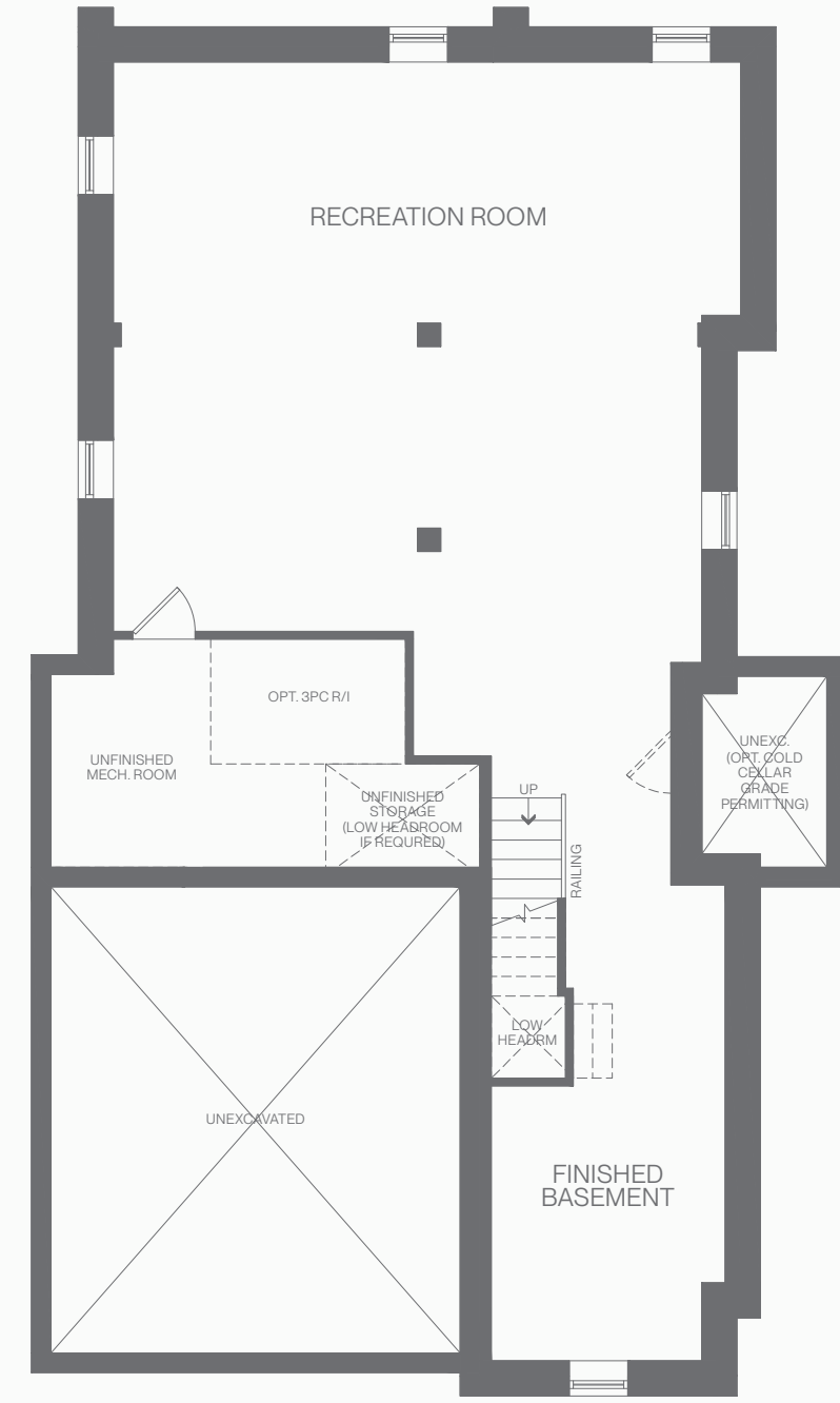
FINISHED BASEMENT PLAN / ELEVATION A
