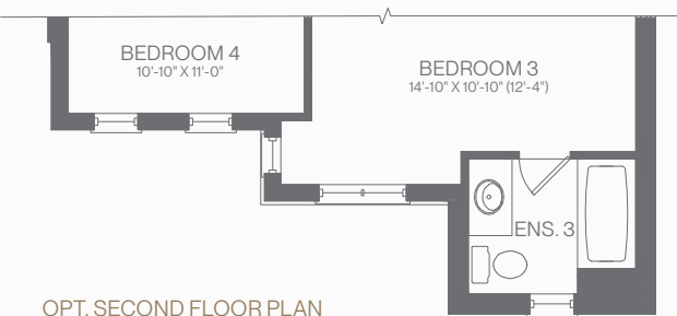
OPT. SECOND FLOOR PLAN
