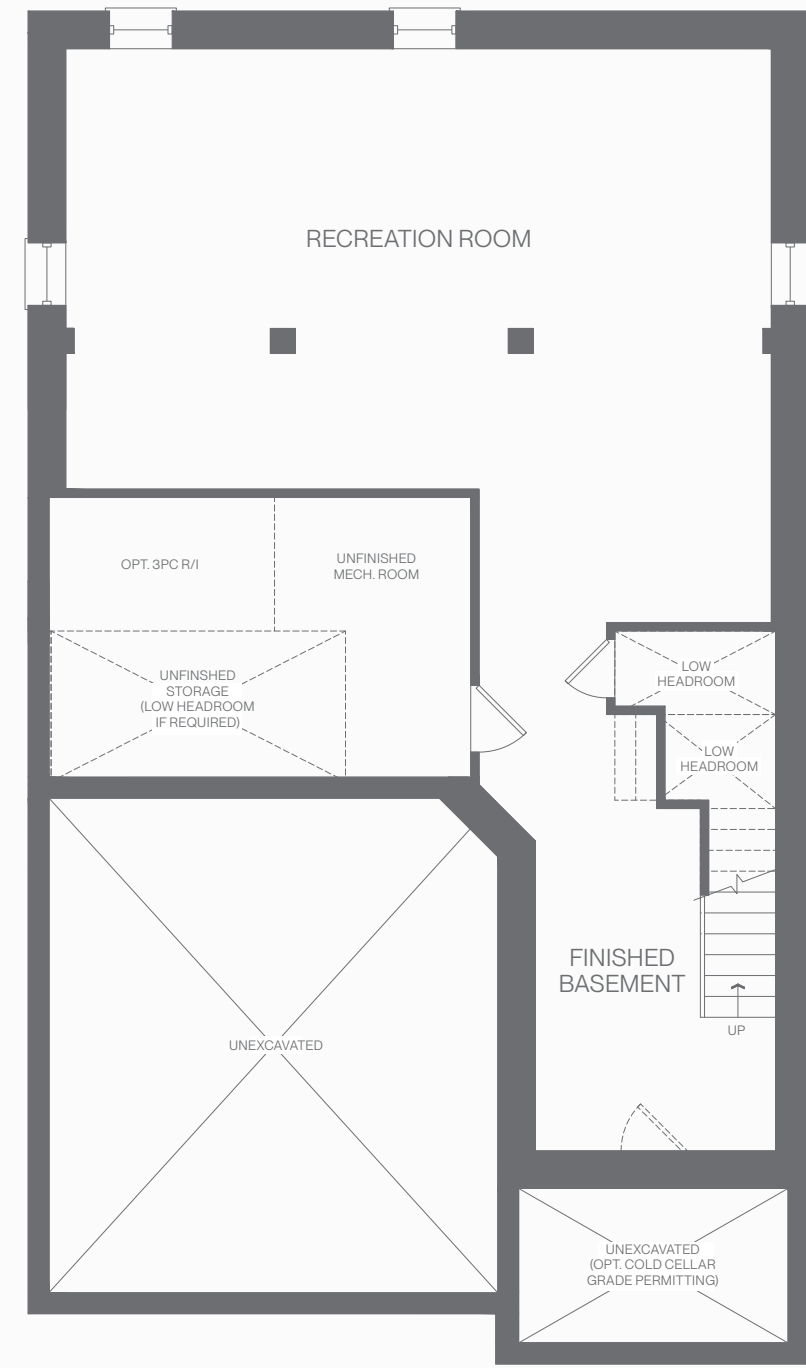
FINISHED BASEMENT PLAN / ELEVATION A + B
