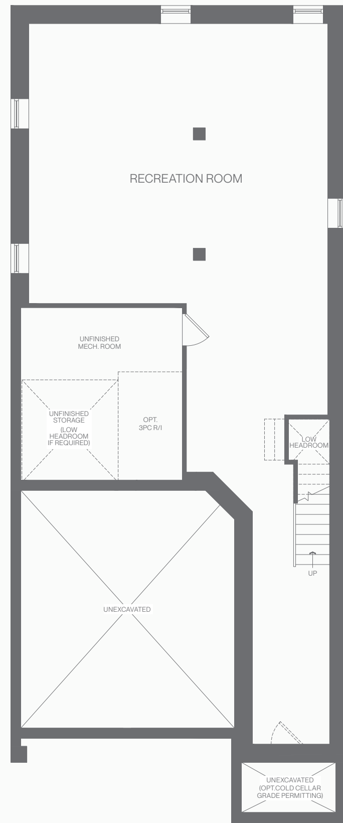
FINISHED BASEMENT PLAN / ELEVATION A, B + C
