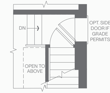
PARTIAL GROUND FLOOR PLAN W/OPT. SIDE DOOR ELEVATION A, B + C
