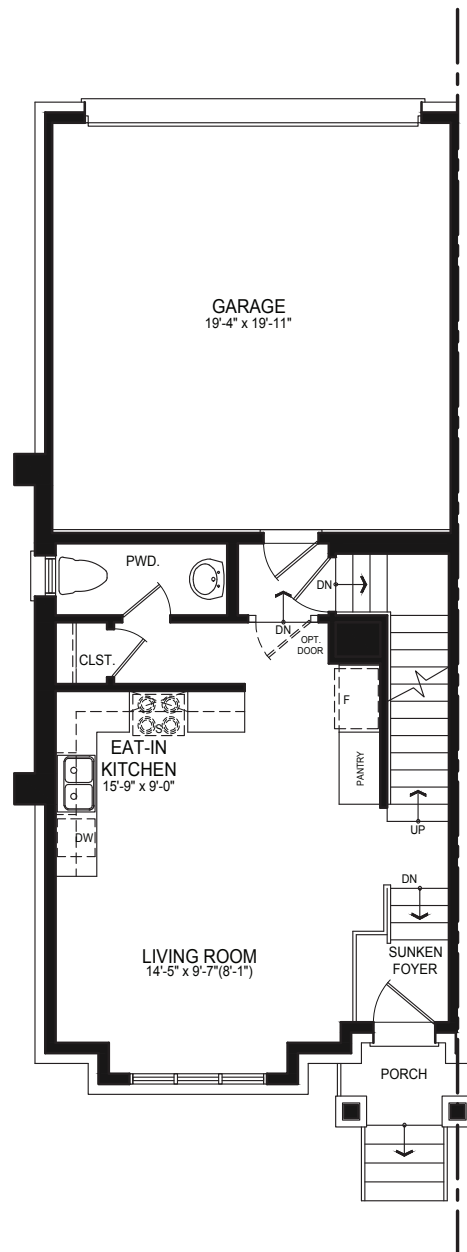
MAIN FLOOR
