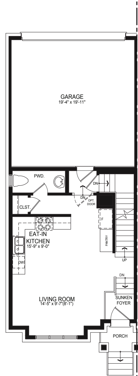
MAIN FLOOR
