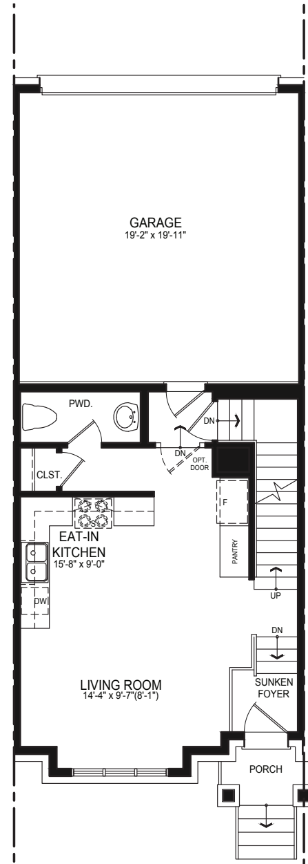
MAIN FLOOR
