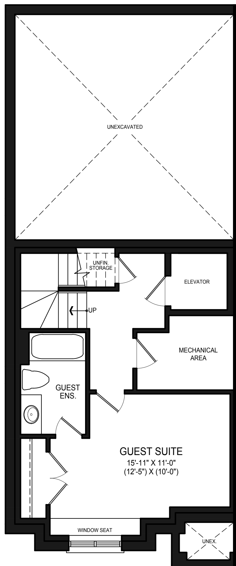
FINISHED BASEMENT PLAN ELEV. A
