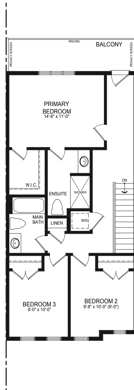
UPPER FLOOR
