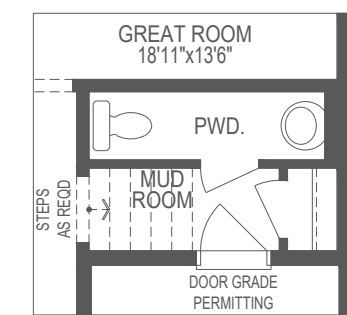
PARTIAL GROUND FLOOR WITH ALTERNATE POWDER ROOM
