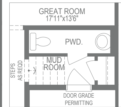
PARTIAL GROUND FLOOR WITH ALTERNATE POWDER ROOM
