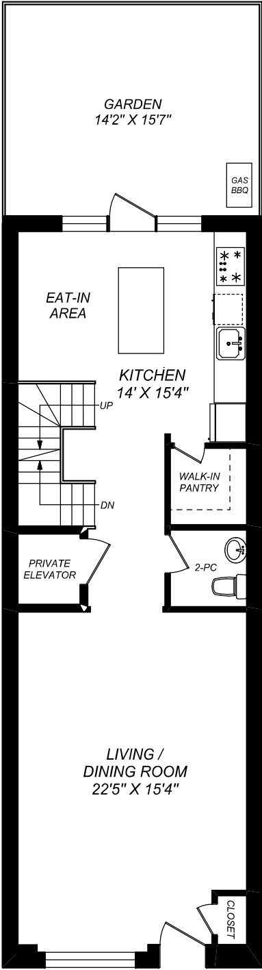
MAIN FLOOR 813 SQUARE FEET (CEILING HEIGHT : 10'-0")
