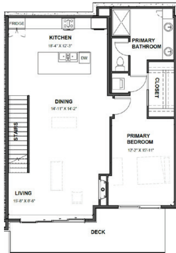
LEVEL 2
