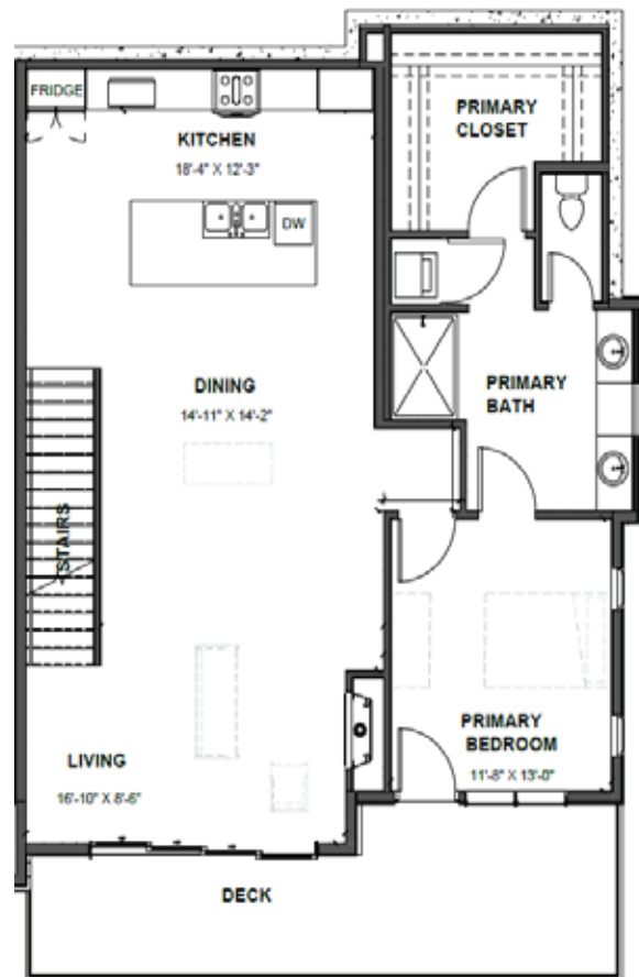
LEVEL 2
