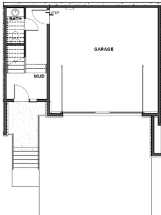
LEVEL 1
