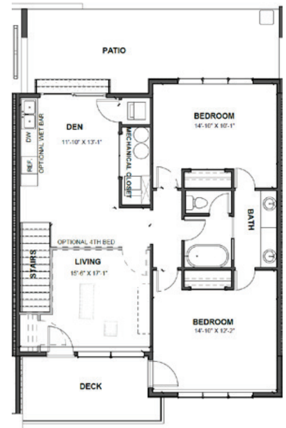
LEVEL 3
