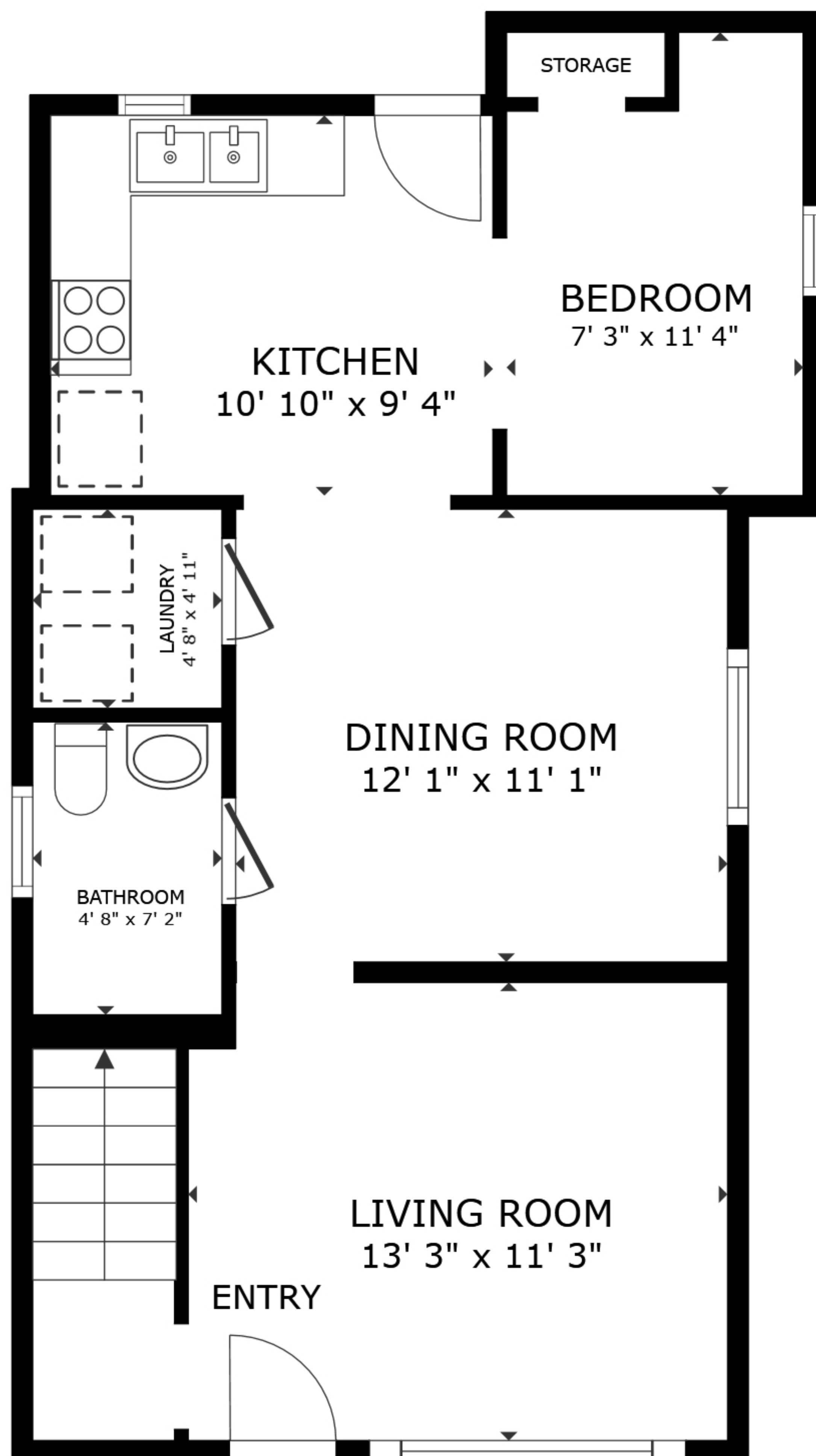
FLOOR 1
