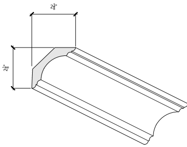
CLASSIC CROWN
