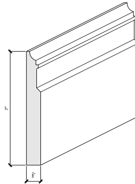
CLASSIC BASE
