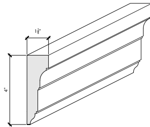
CLASSIC CASING
