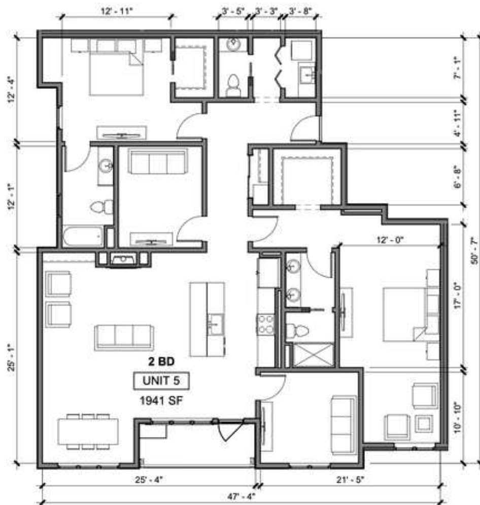
1 UNIT 5 - ENLARGED PLAN A2.13 SCALE: 1/8" = 1'-0"
