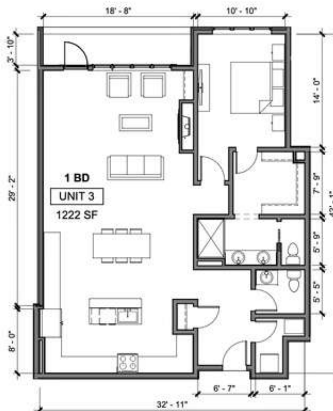
1 UNIT 3 - ENLARGED PLAN A2.12 SCALE: 1/8" = 1'-0"
