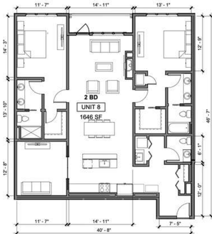
2 UNIT 8+12 - ENLARGED PLAN A2.14 SCALE: 1/8" = 1'-0"
