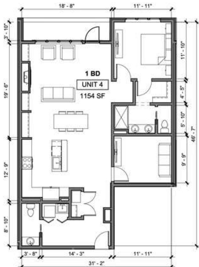
2 UNIT 4 - ENLARGED PLAN A2.12 SCALE: 1/8" = 1'-0"
