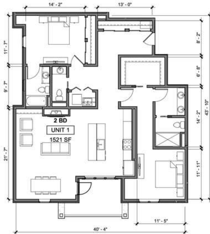
1 UNIT 1 - ENLARGED PLAN A2.11 SCALE: 1/8" = 1'-0"
