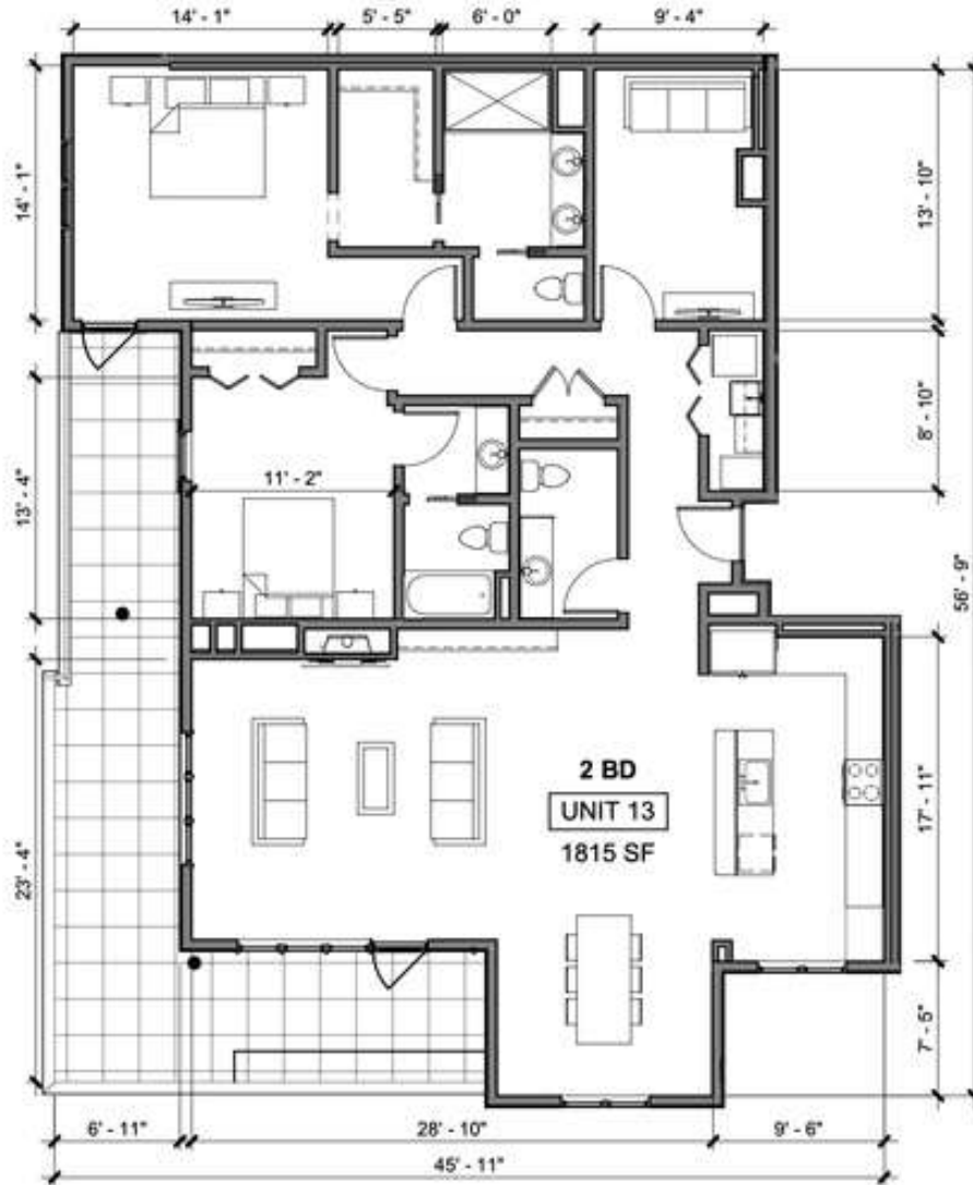
1 UNIT 13 - ENLARGED PLAN
