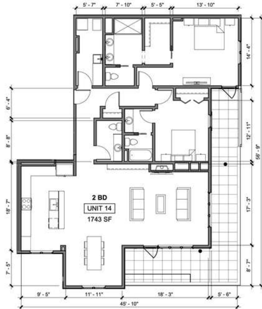
2 UNIT 14 - ENLARGED PLAN
