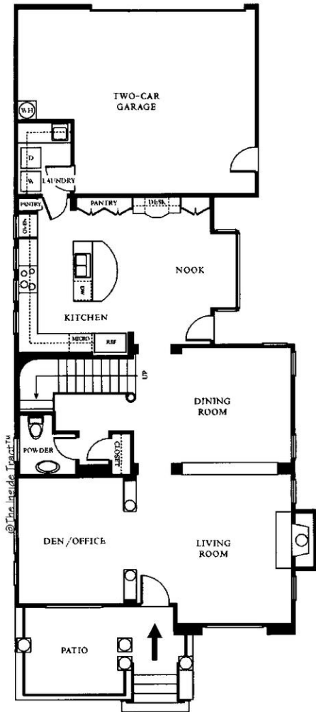
First Floor
