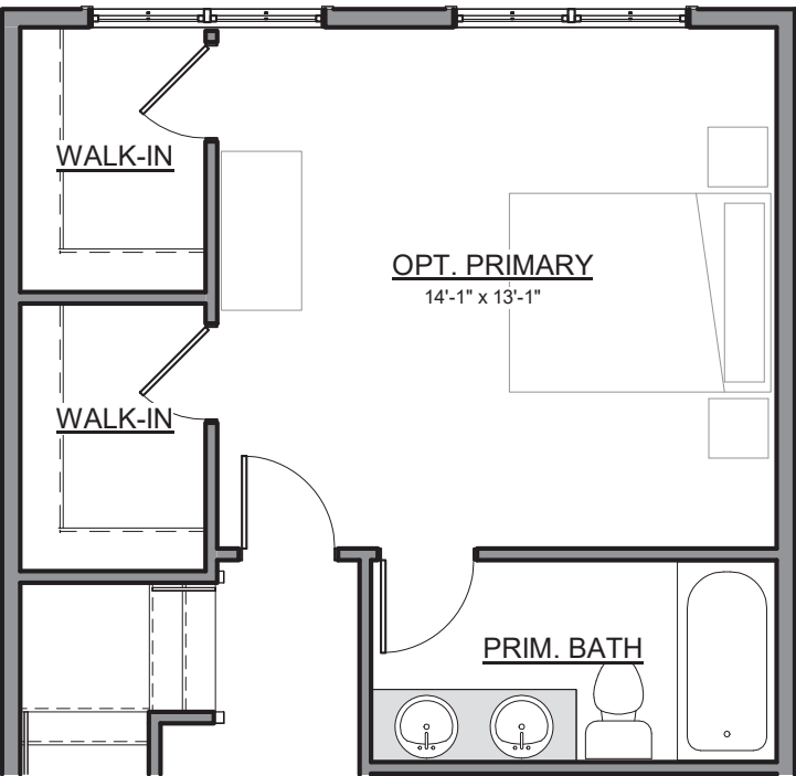
OPT. PRIMARY SUITE UNITS 1-5, 12-16
