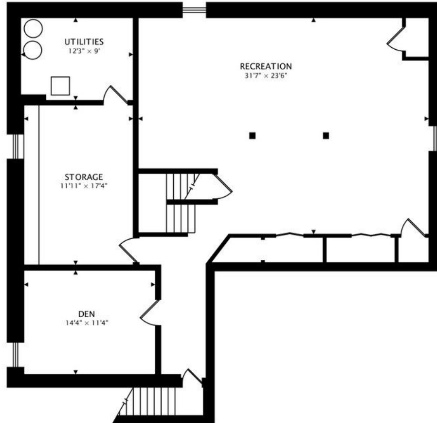
LOWER 1665 sq ft BELOW GRADE
