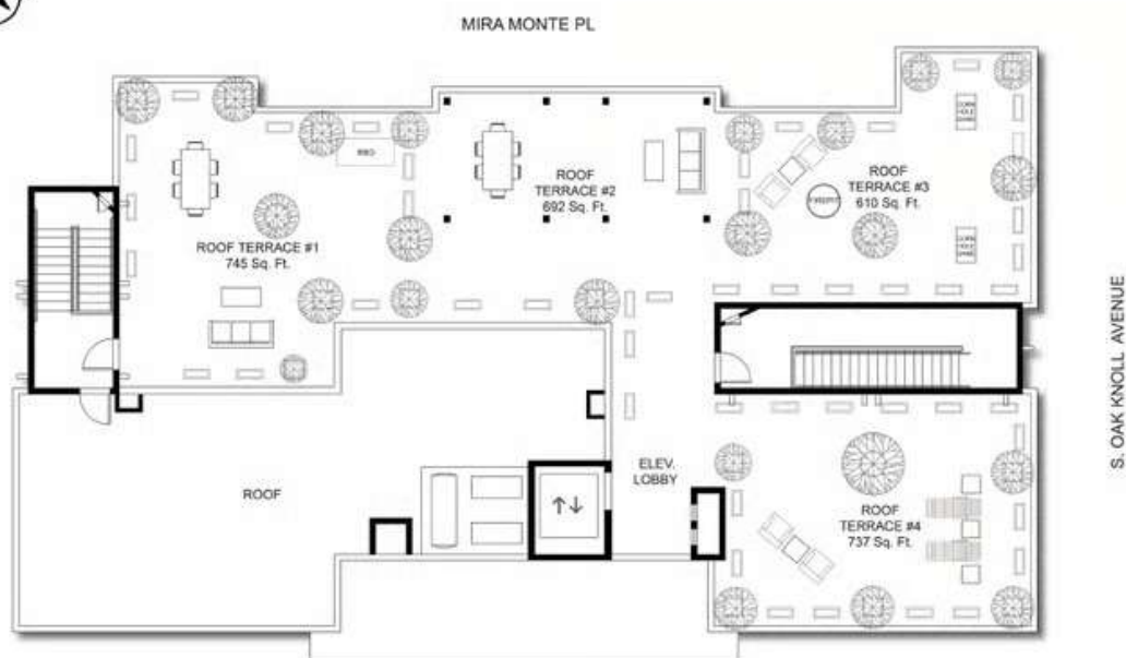
5TH/ROOF LEVEL FLOOR PLAN
