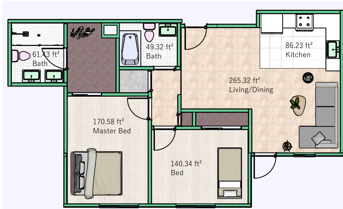
FLOOR PLAN 2D 2 BEDROOM, 2 BATH UNIT 104, 204, 304 & 404
