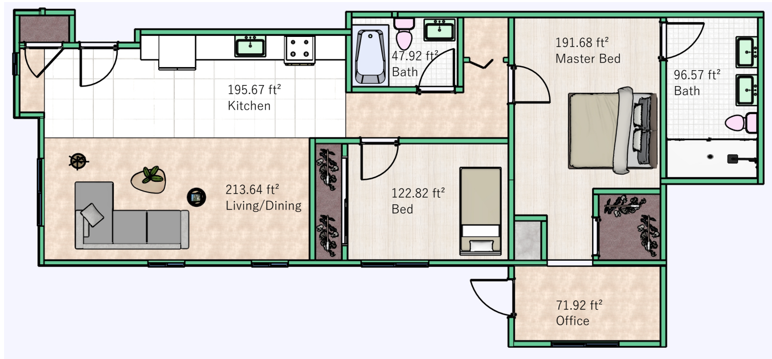
FLOOR PLAN 2B 2 BEDROOM, 2 BATH UNIT 202, 302 & 402
