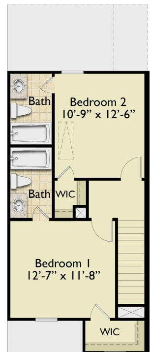
SECOND FLOOR
