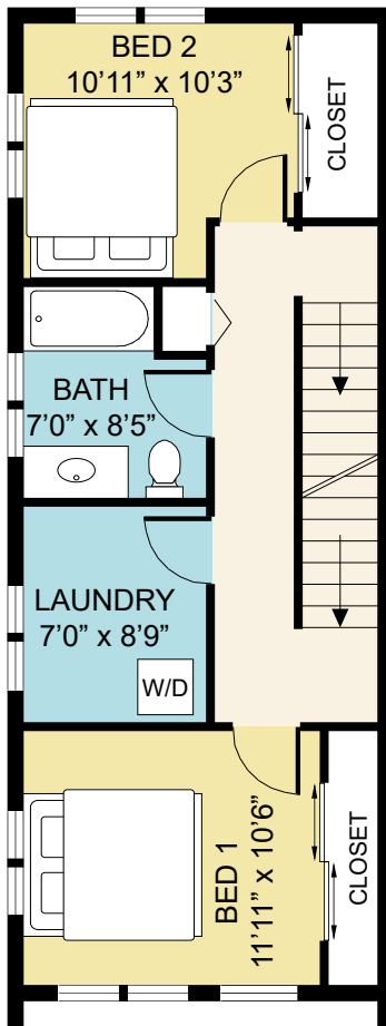
SECOND FLOOR
