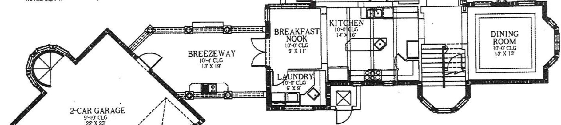
GROUND FLOOR PLAN 2236 A.C. SQ. FT.
