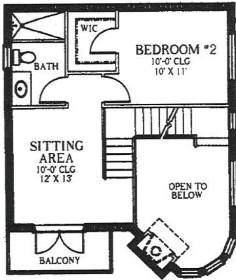
SECOND FLOOR PLAN 620 A.C. SQ. FT.
