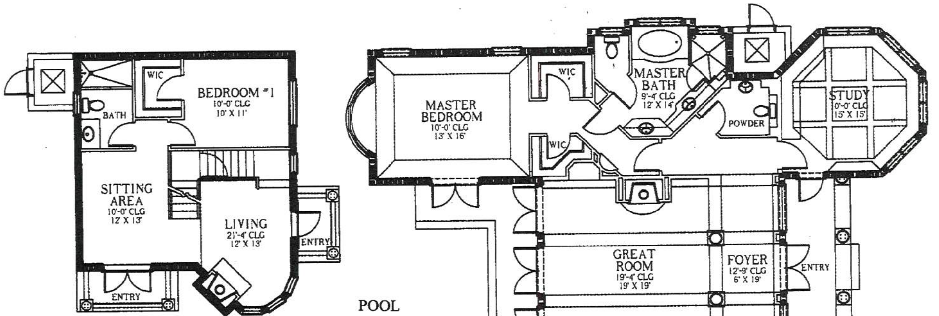
GROUND FLOOR PLAN 413 A.C. SQ. FT.
