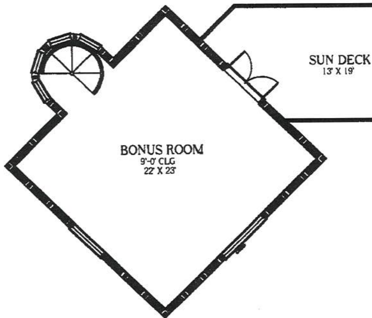
SECOND FLOOR PLAN 620 A.C. SQ. FT.
