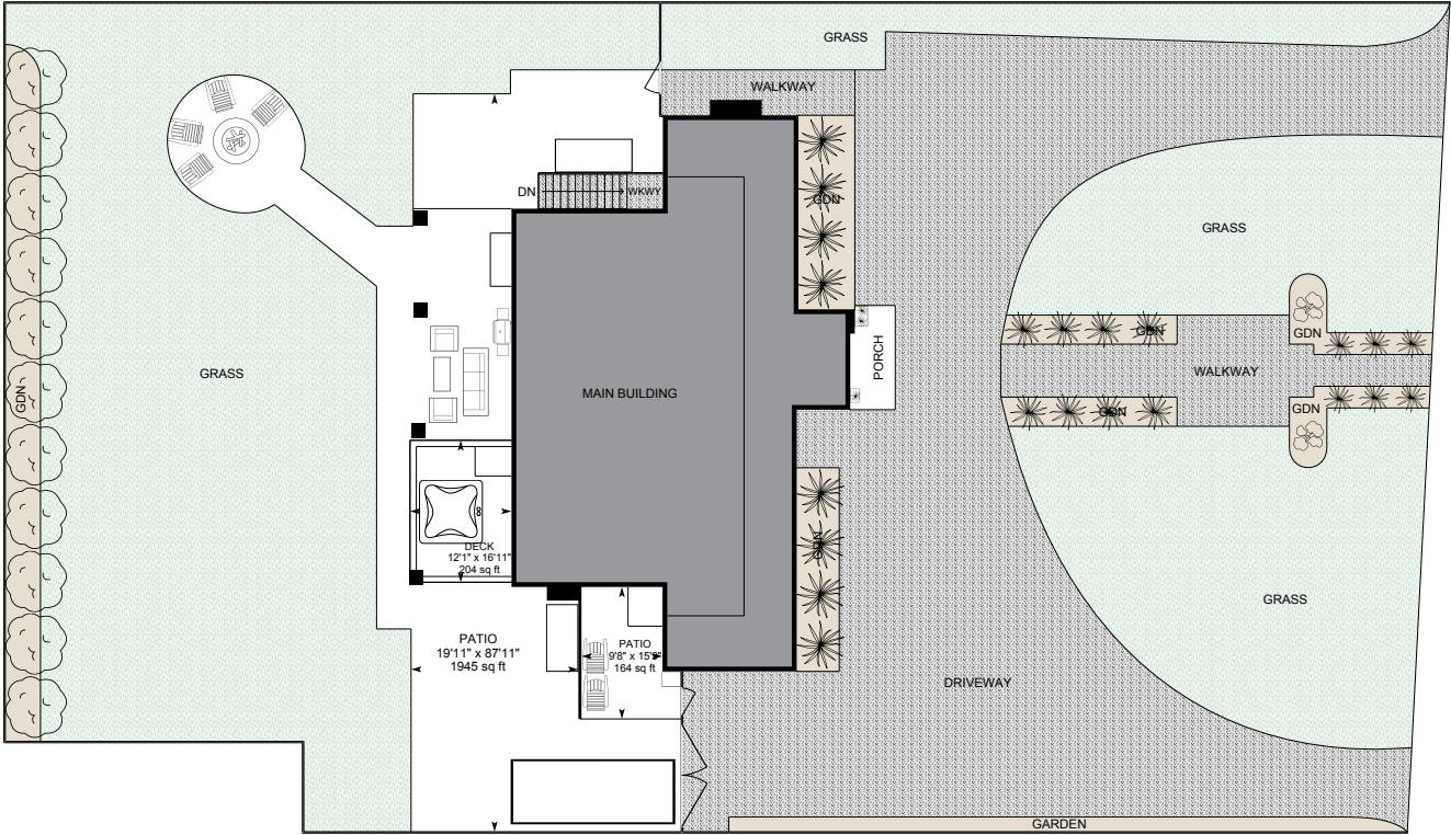
Site Plan
