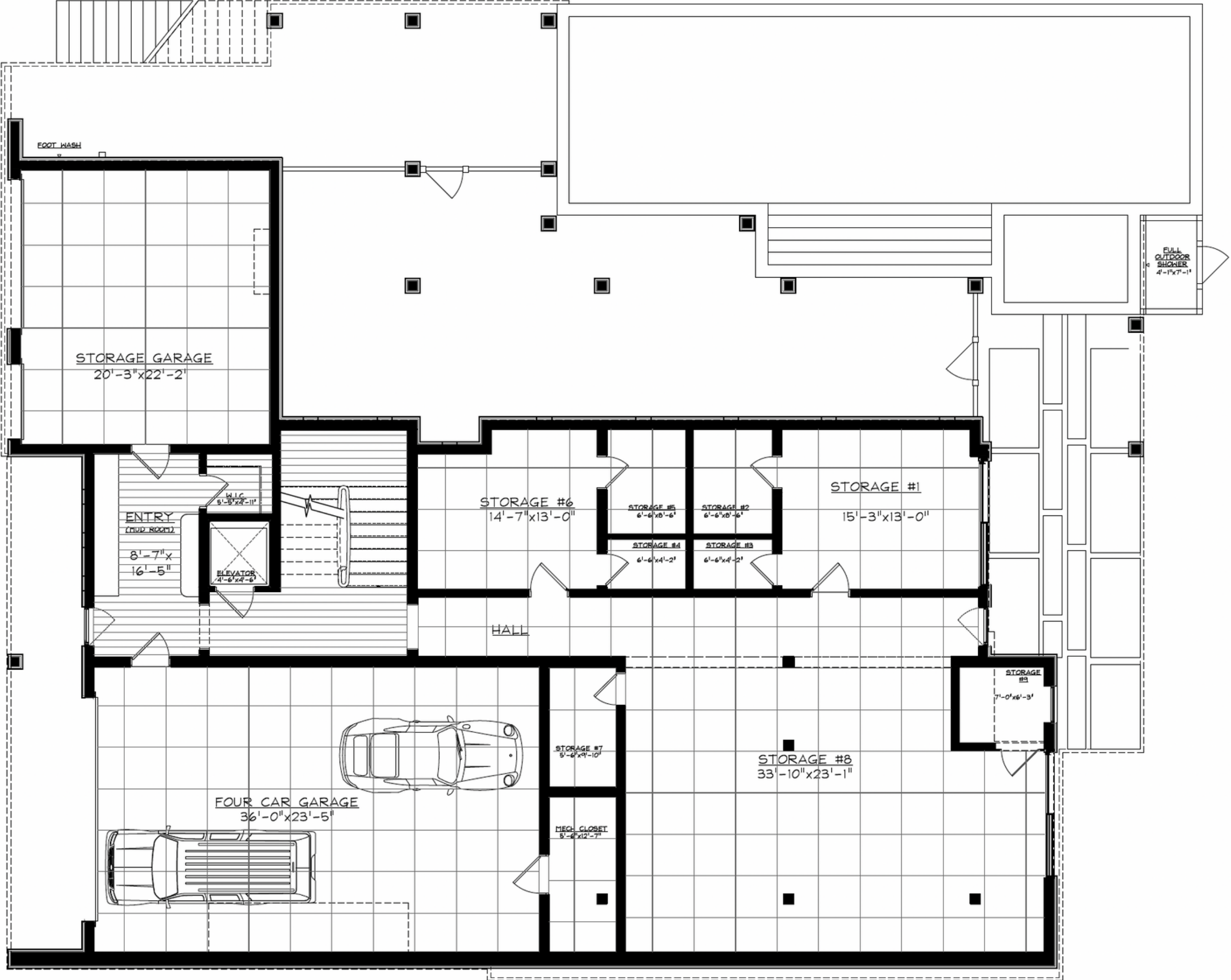
GROUND FLOOR PLAN (12-03-25) 125 DUNE ROAD
