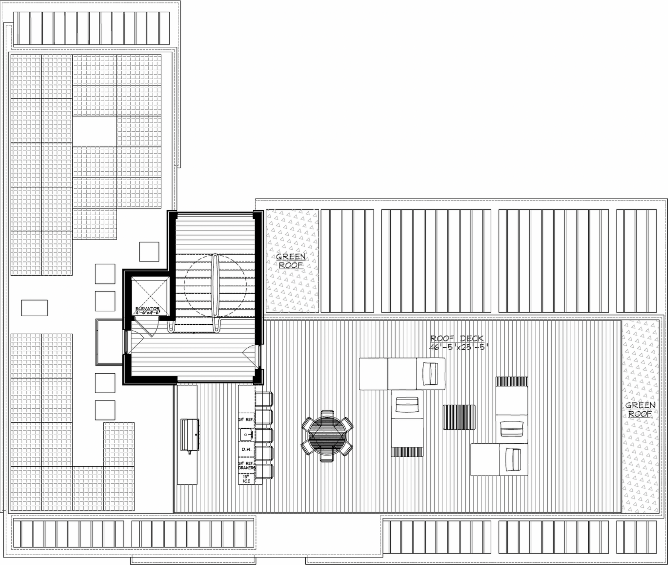
ROOF PLAN (12-03-25) 125 DUNE ROAD
