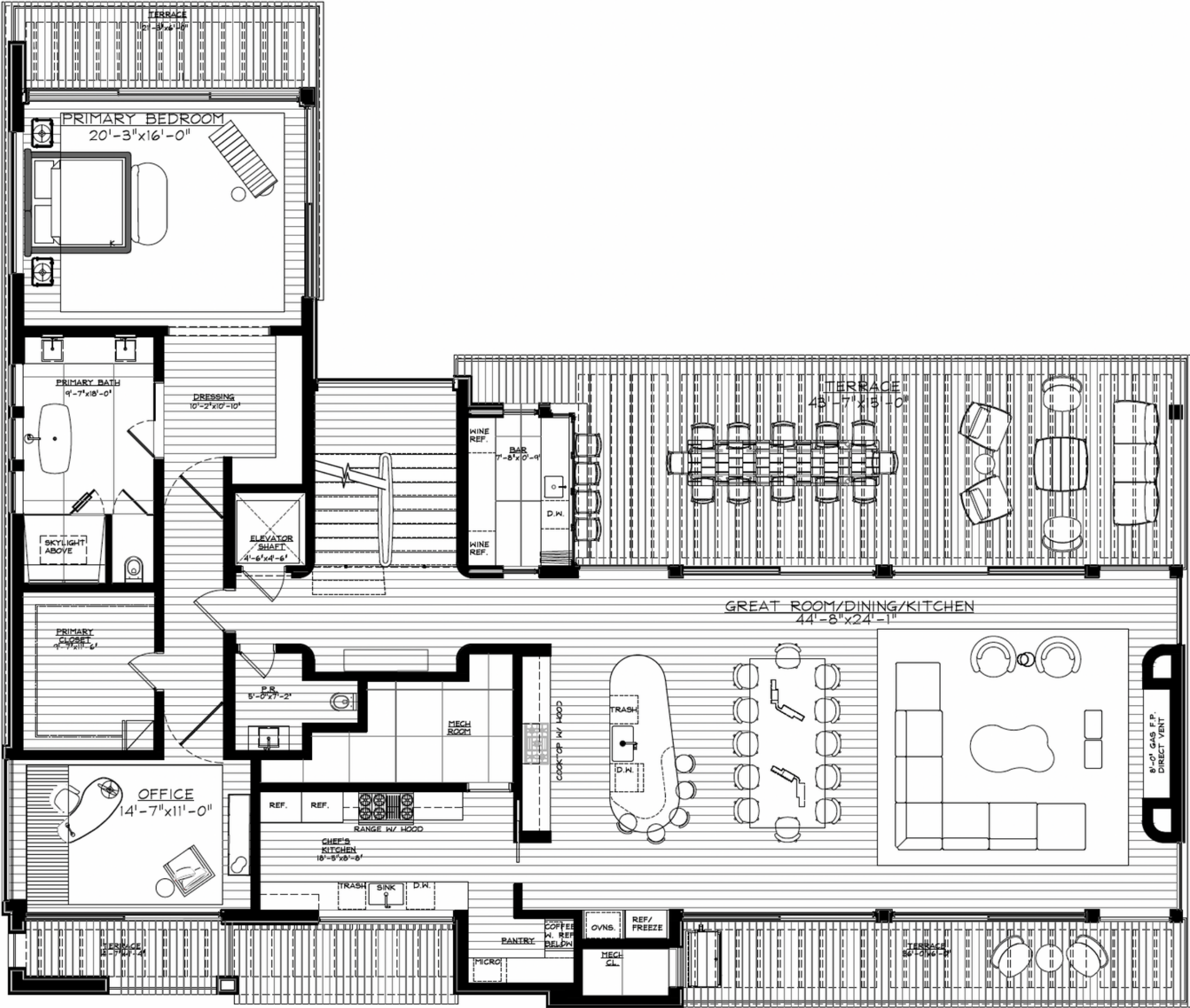
SECOND FLOOR PLAN (12-03-25)
