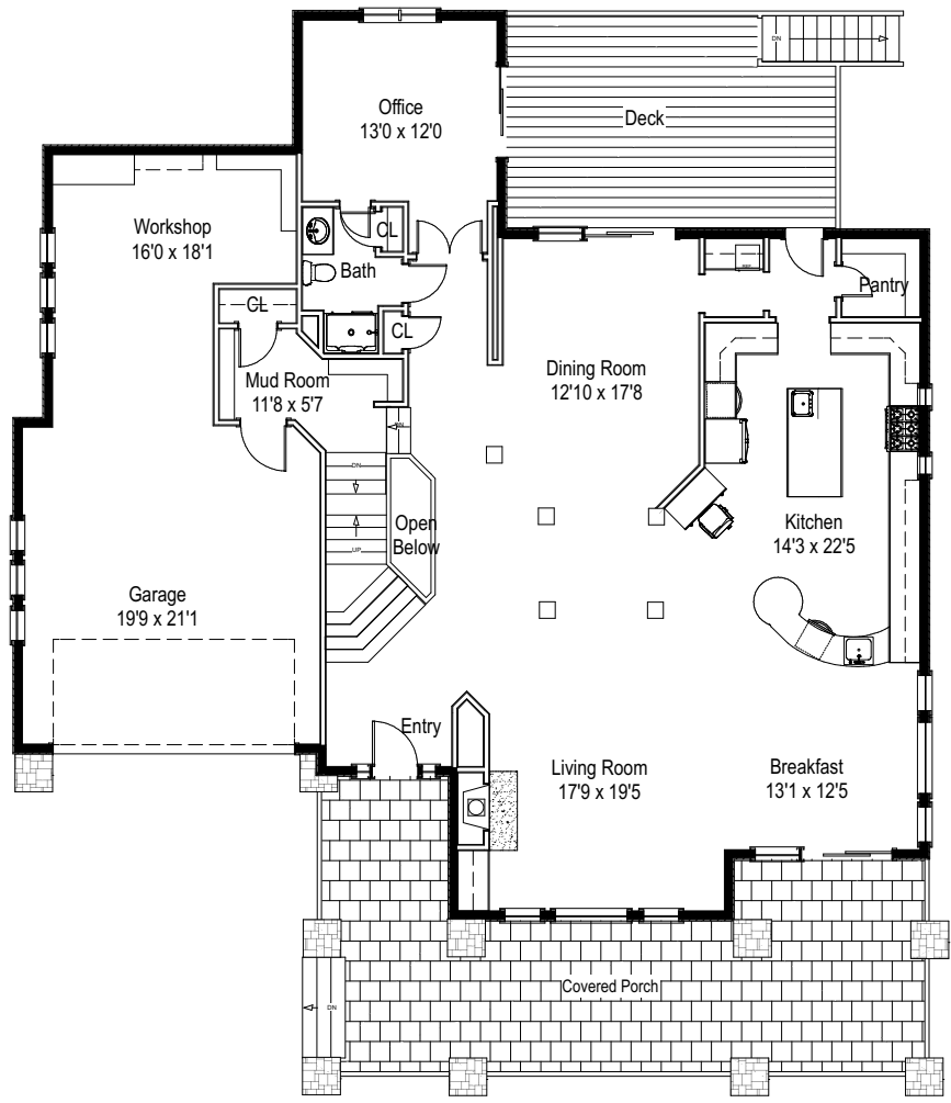
Main Level - 1985 square feet +/-
