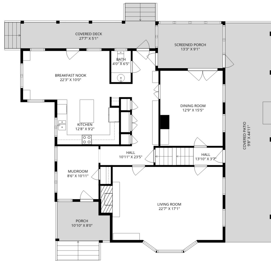
1ST FLOOR
