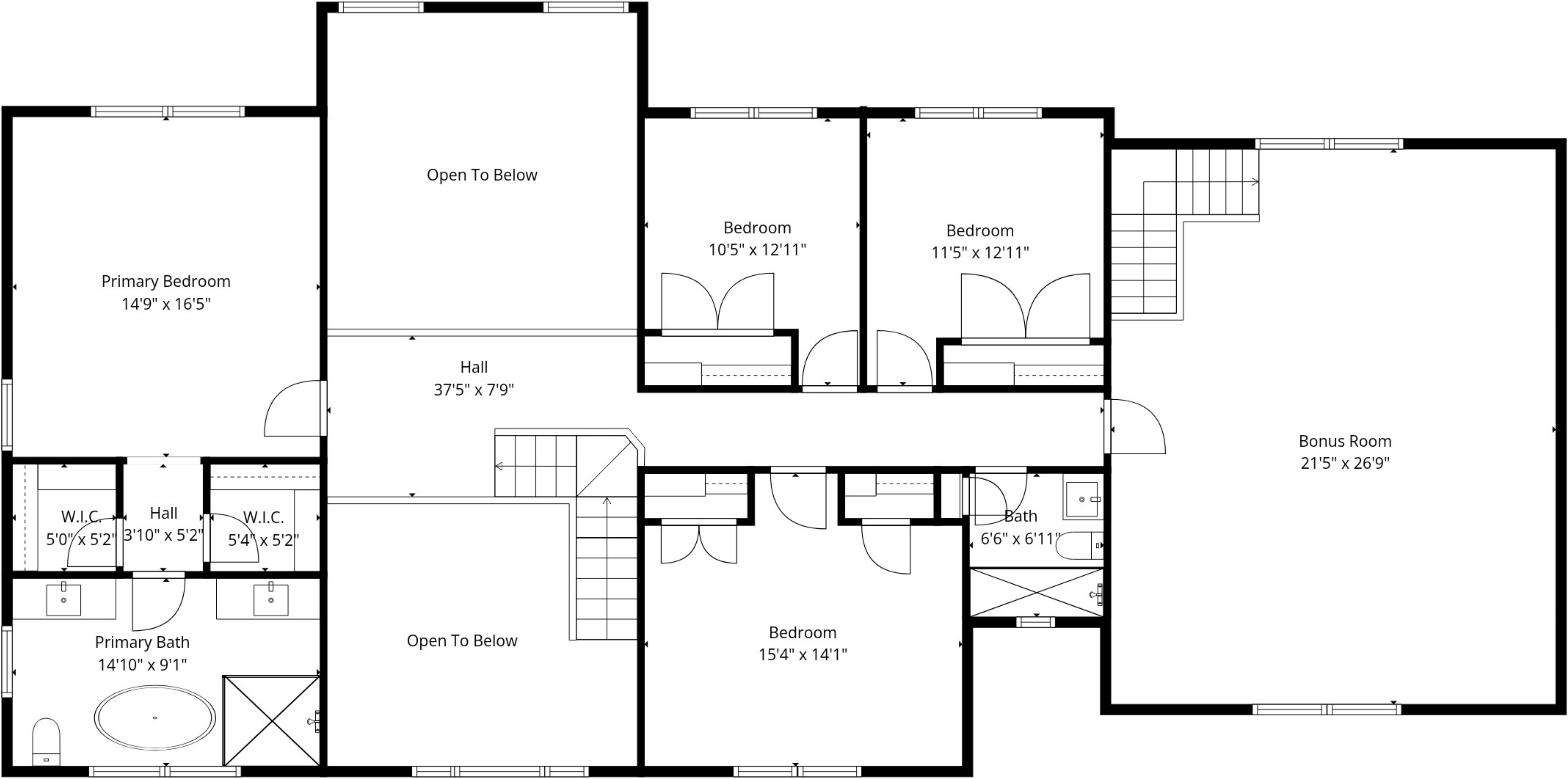
Floor 3
