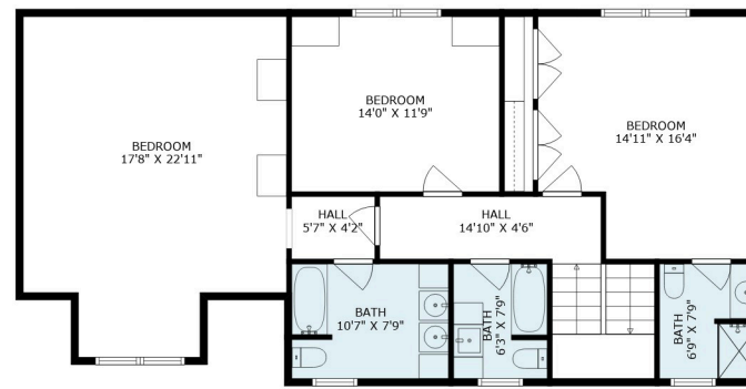
FLOOR 3
