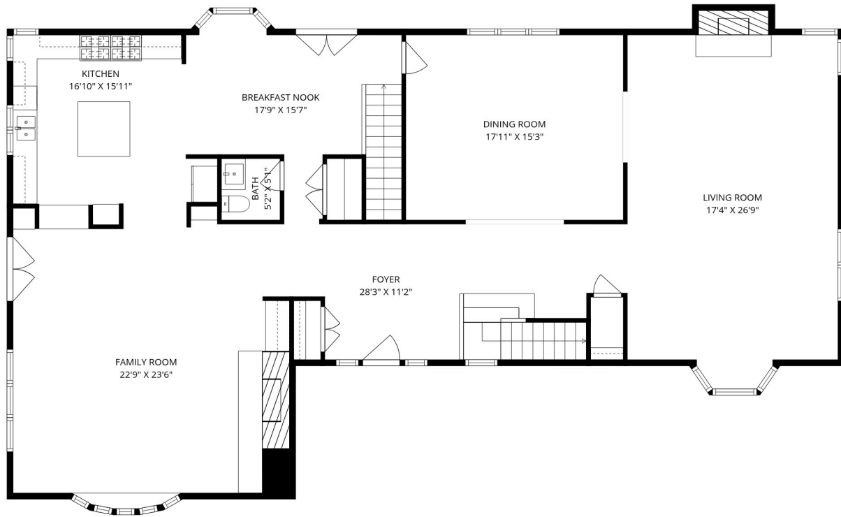
1ST FLOOR
