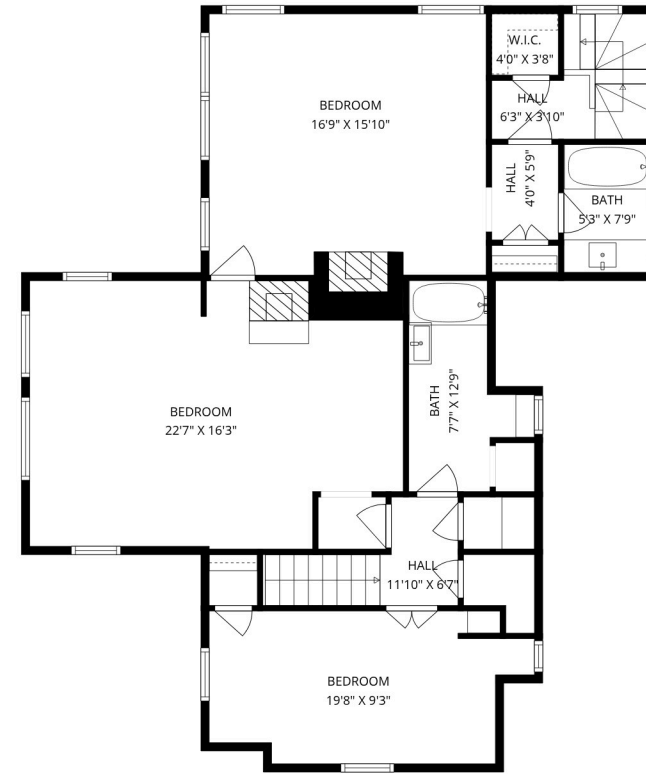
2ND FLOOR
