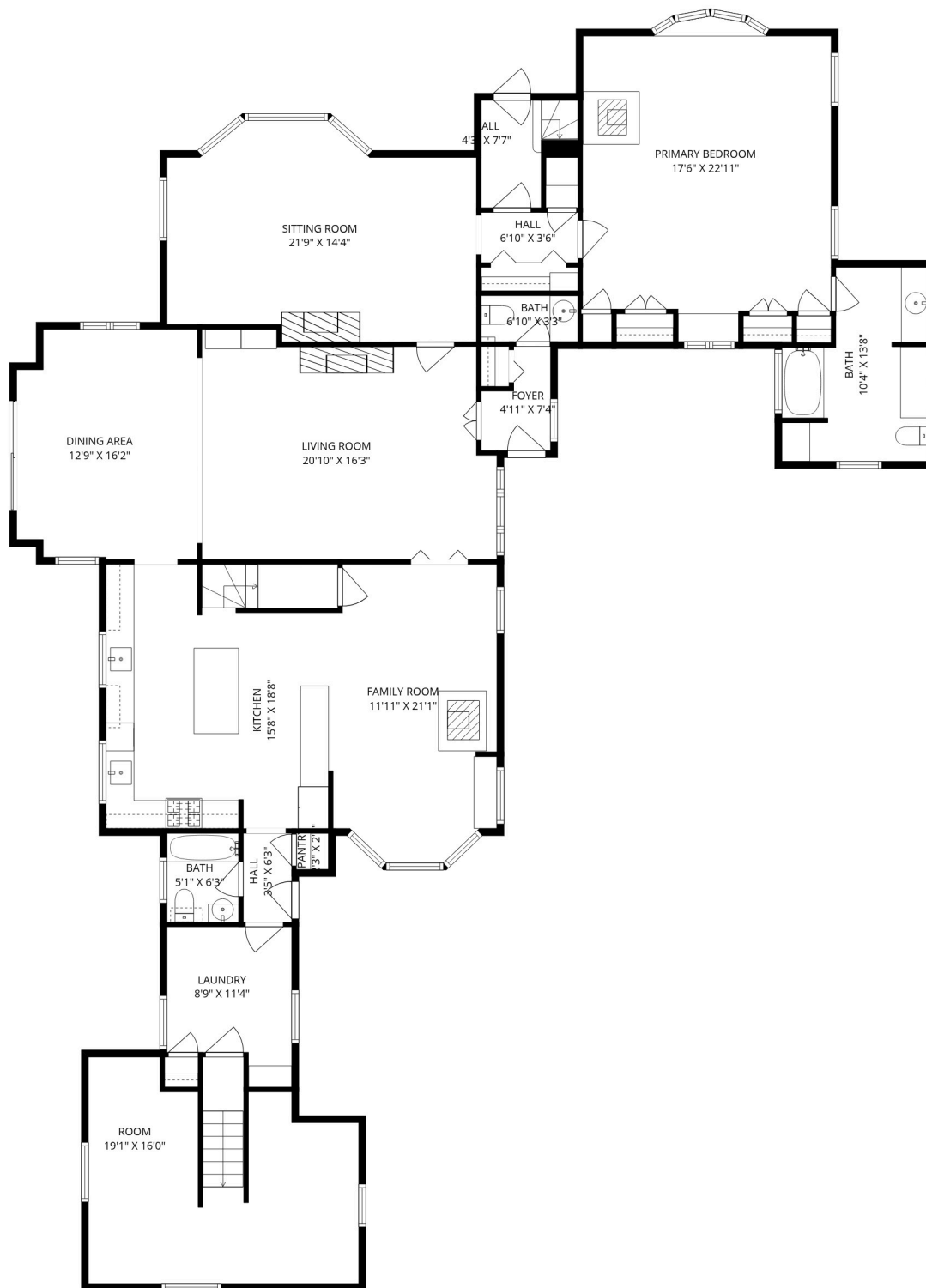
1ST FLOOR
