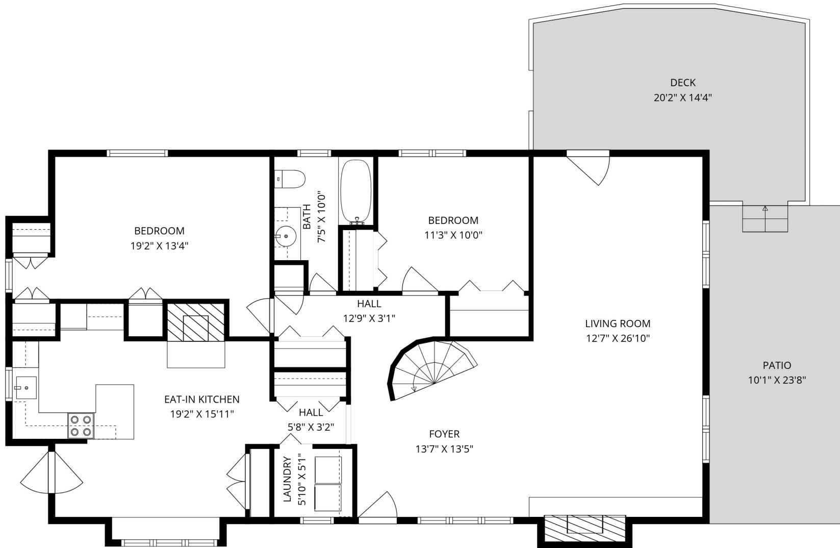
1ST FLOOR
