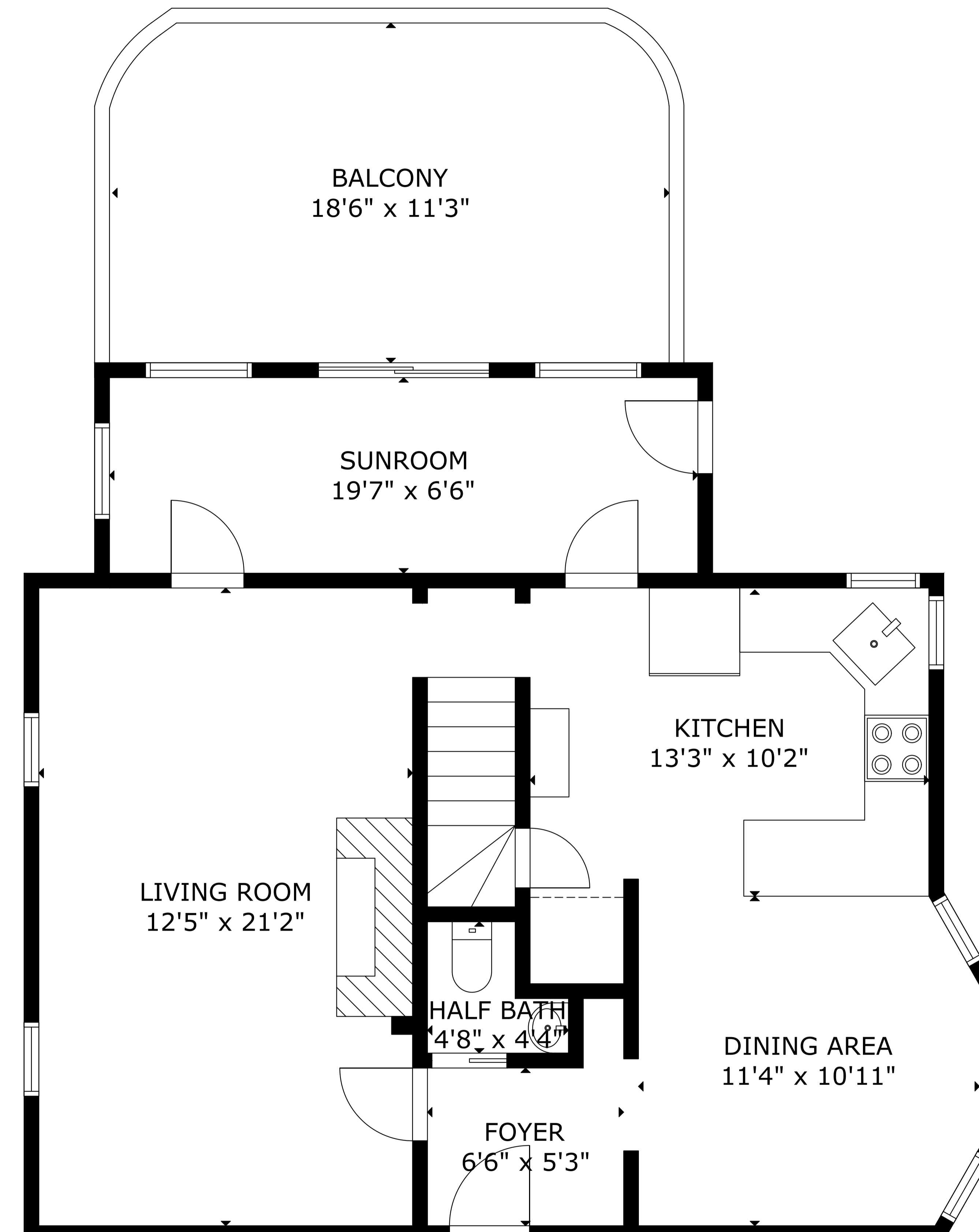
FLOOR 1
